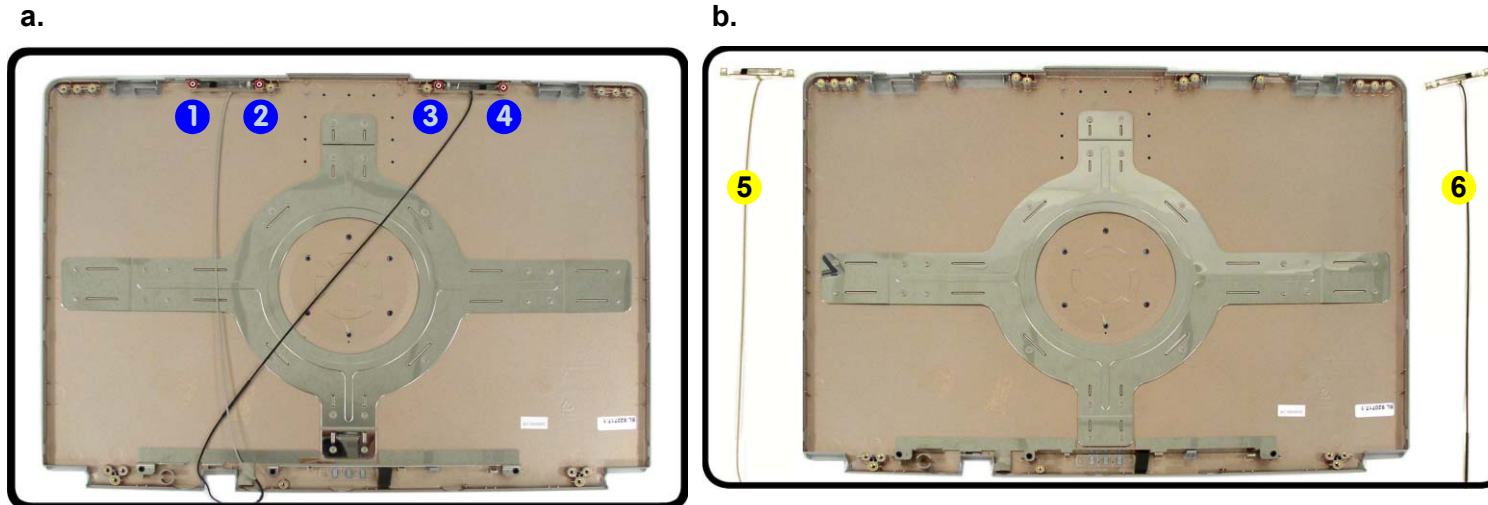
Figure 24 Bluetooth & WLAN Antenna Removal
