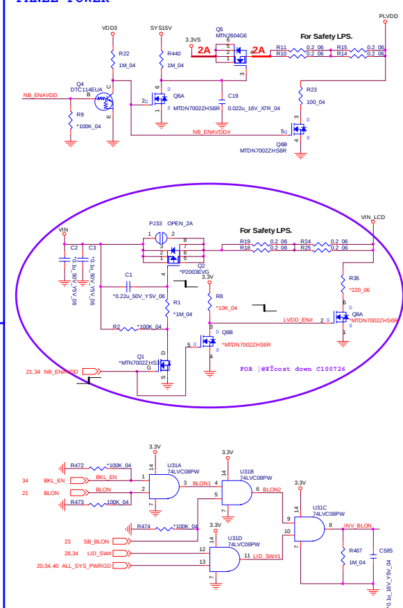
PANEL POWER
