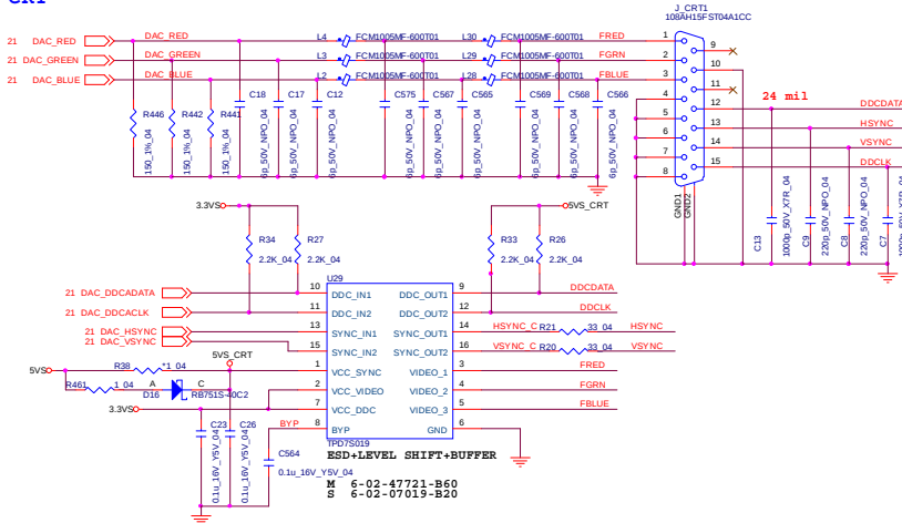
CRT
