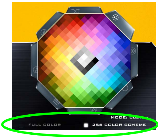
Figure 8 - Color Swatch
