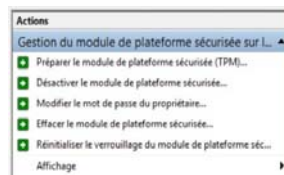
Figure 35 Menu Actions
