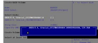
Figure 4 - Select Disks
