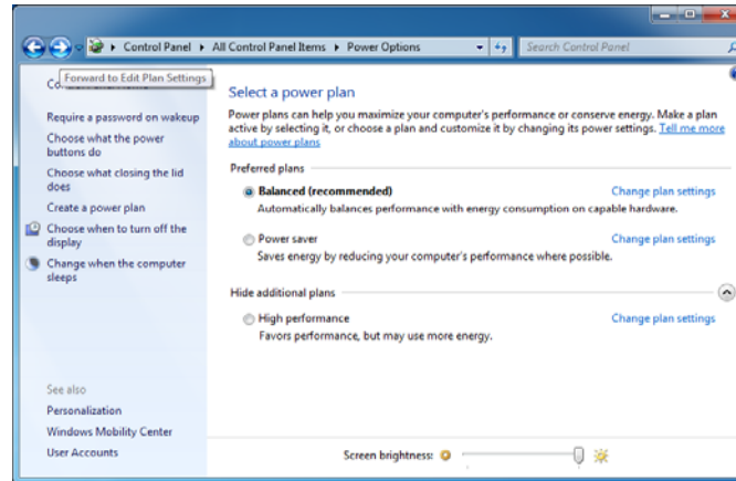
Figure 31 - Power Options
