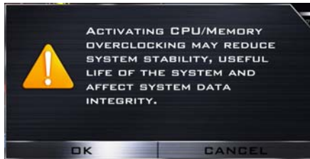
Figure 15 - CPU Overclocking
