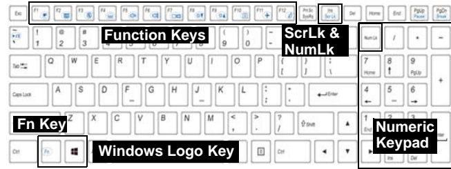
Figure 6 - Keyboard
