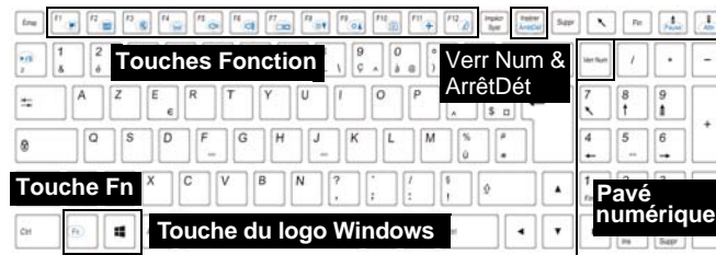
Figure 6 - Clavier
