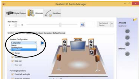
Figure 29 Speaker Configuration
