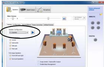
Figure 28 Speaker Configuration
