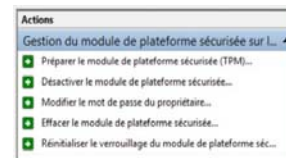
Figure 34 Menu Actions
