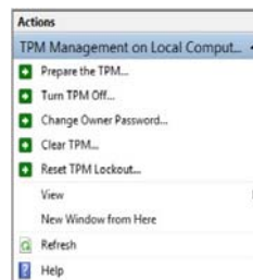
Figure 34 Actions Menu
