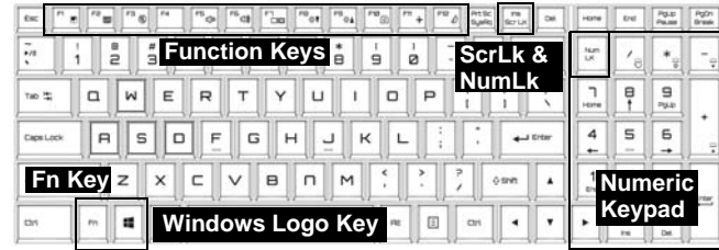
Figure 5 - Keyboard
