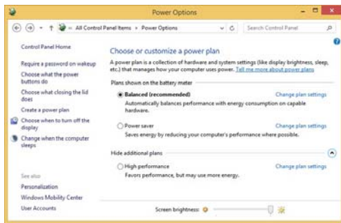
Figure 27 - Power Options
